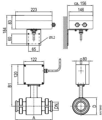
DIN11851, Wandmontage
