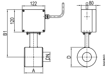
Wandmontage
