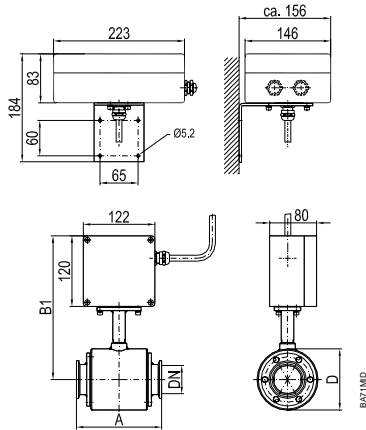
TriClamp®, Wandmontage
