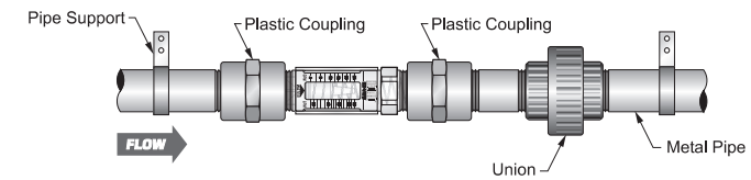
Figure 2: 1 in. (25 mm) NPT model installation
