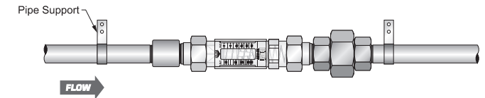
Figure 5: All models with male, metal or PVC threaded end fittings installation
