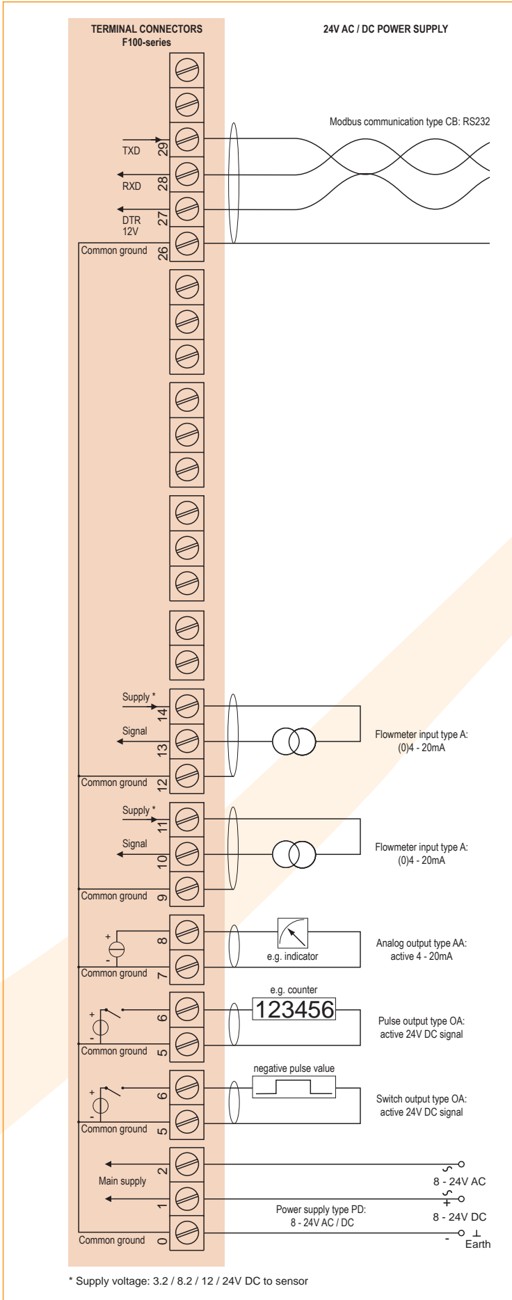
Typical wiring diagram F116-A-AA-CB-OA-PD
