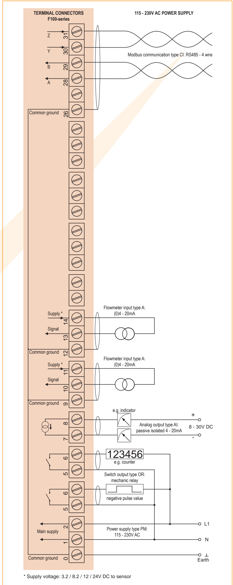
Typical wiring diagram F116-A-AI-CI-OR-PM
