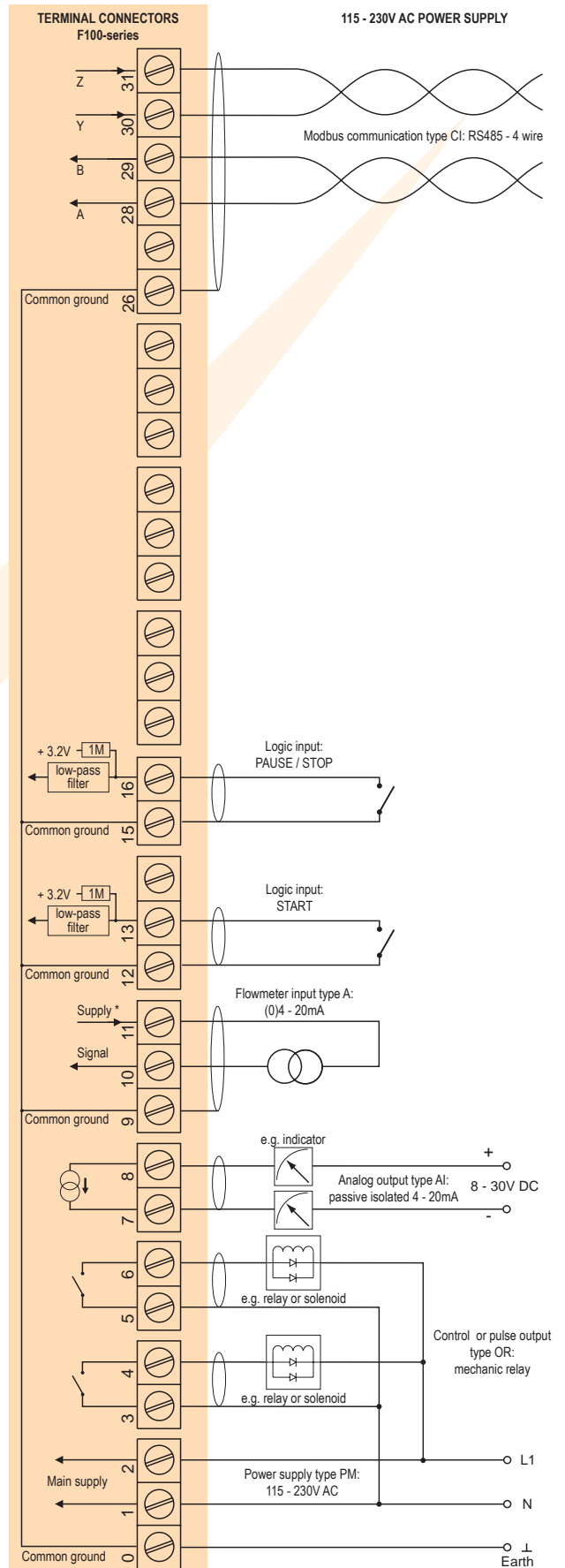
Typical wiring diagram F131-A-AI-CI-OR-PM
